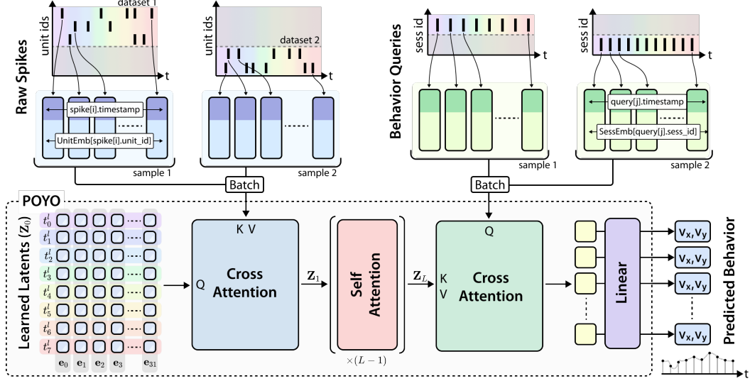
Figure 1: Overview of our approach. Input spike tokens are compressed into a smaller set of latent tokens which are processed through multiple self-attention blocks, finally time-varying outputs are predicted by querying the latent space. All tokens in this model are assigned a timestamp, which are used towards rotary position encoding.
