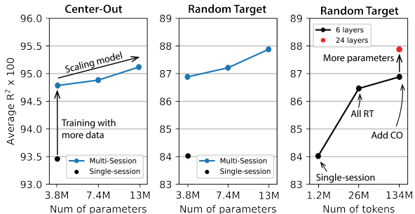
Figure 3: Scaling curves. R^2 is evaluated and averaged over the test splits on both CO and RT tasks. The single-session performance is the mean over 100 different models.
